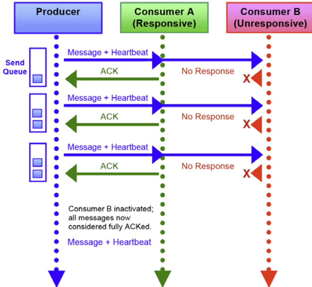
Figure 2: Slow consumer inactivated to clear send queue
