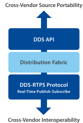
Figure 3. DDS Connectivity Model
